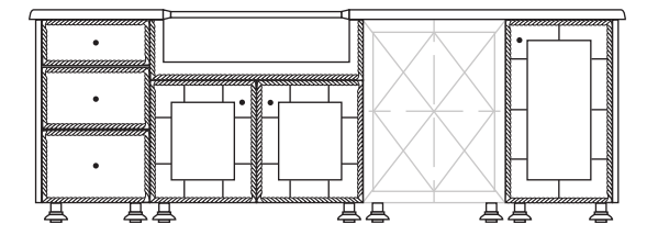
Drawer Cabinet, Appliance Opening Panel and Door Cabinet
